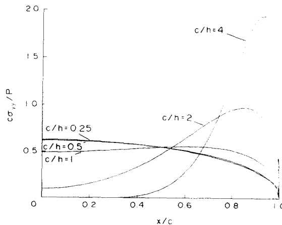
Fig. 3. Contact stresses for L/h = 10 and clamped ends.
